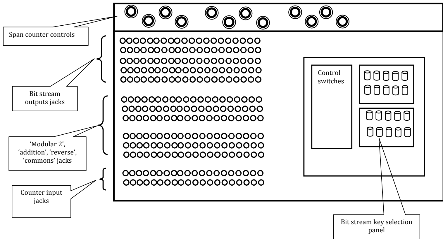
Schematic diagram of Colossus 6 'set up' panel
